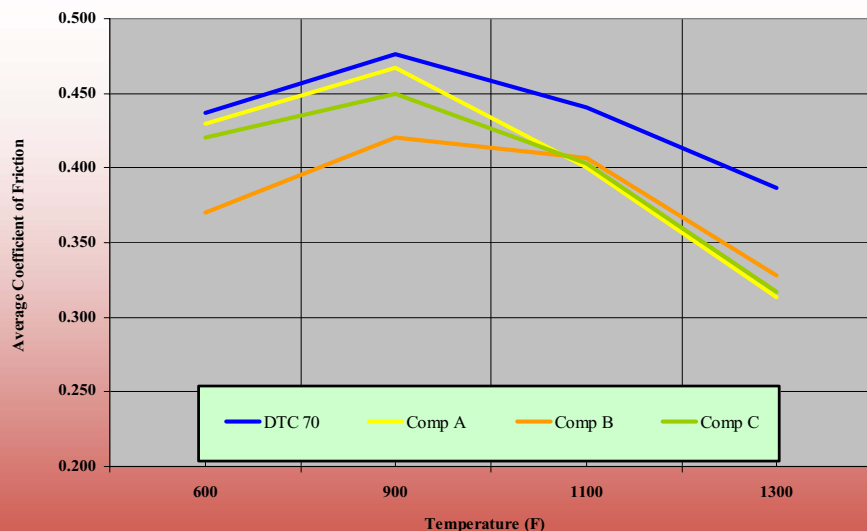
NASCAR Simulation Performance vs. Temperature
