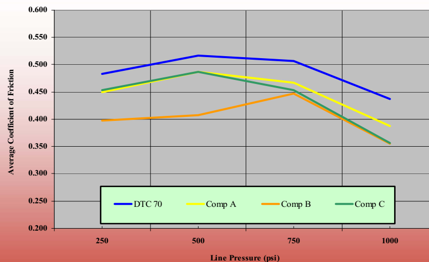
NASCAR Simulation Performance vs. Pressure
